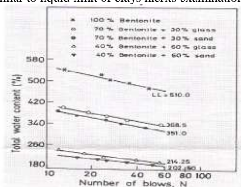
Fig 2 Flow lines for Bentonite and Bentonite sand or glass Particle mixtures
