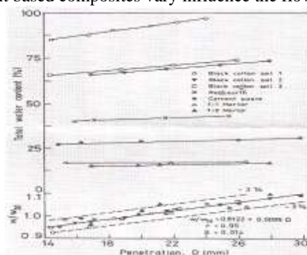
Fig.1 Flow lines of clays and cement based materials & their Normalization (Nagaraj et al 1989)
